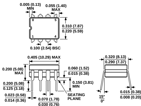
Figure 36. 8-Lead Ceramic Dual In-Line Package [CERDIP]
