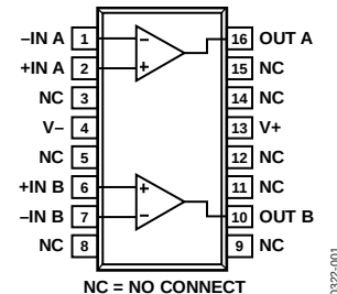
Figure 1. 16-Lead SOIC (S-Suffix)
