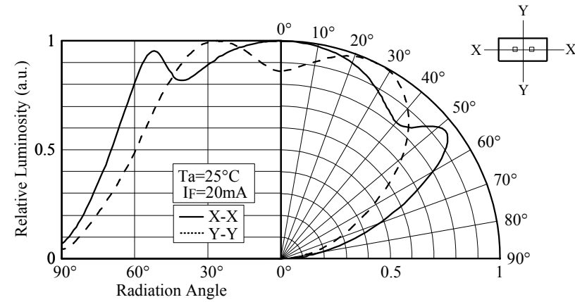
■ Directivity (NSPWF50BS)
