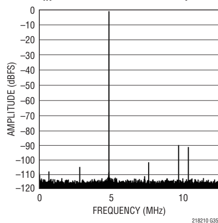
LTC2180: 64k Point FFT, f_{IN} = 70\text{MHz} , -1dBFS, 25MSPS
