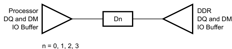
Figure 9-75. DQ/DM Topology
