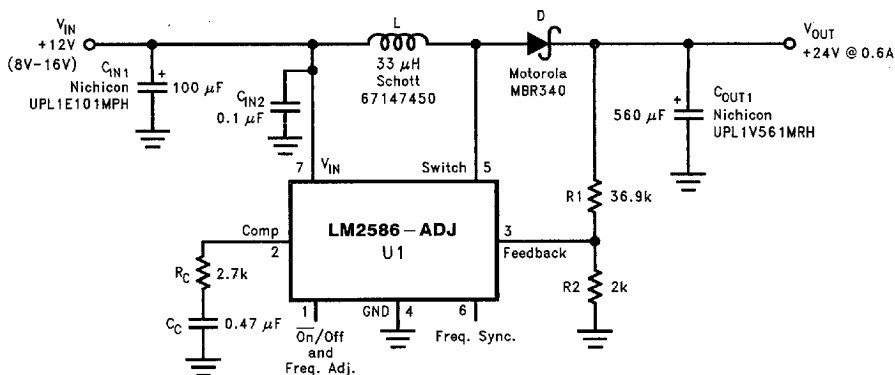
FIGURE 35. +12V to +24V Boost Regulator
