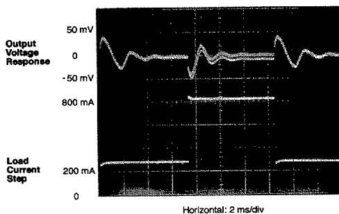
FIGURE 6. V_{OUT} Response to Load Current Step
