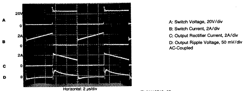
FIGURE 5. Switching Waveforms
