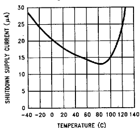
Shutdown Supply Current vs Temperature
