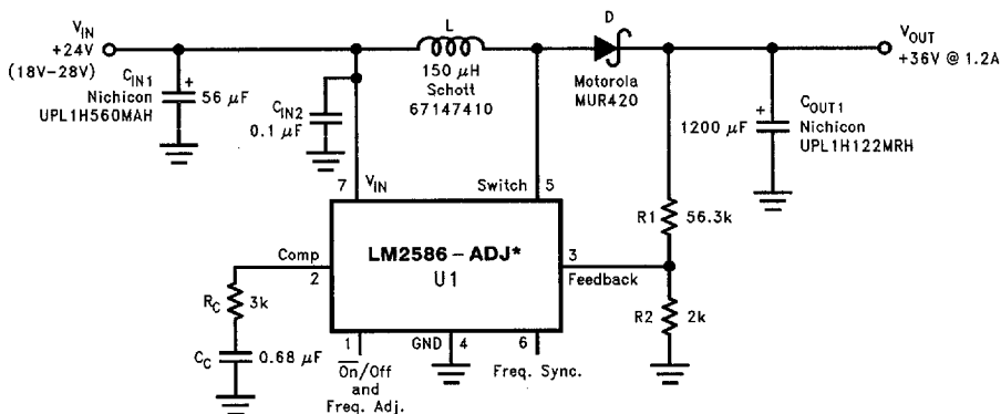
FIGURE 36. +24V to +36V Boost Regulator
