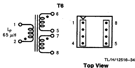
FIGURE 16. Coilcraft Q4339-B
