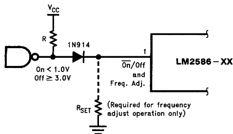
FIGURE 38. Shutdown Operation
