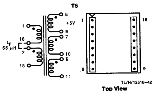
FIGURE 23. Pulse PE-68413 (Surface Mount)
