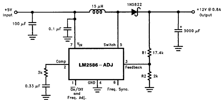
FIGURE 42. Boost Regulator
