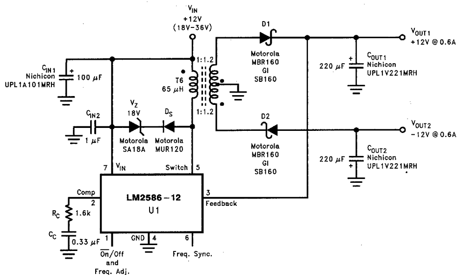
FIGURE 11. Dual-Output Flyback Regulator
