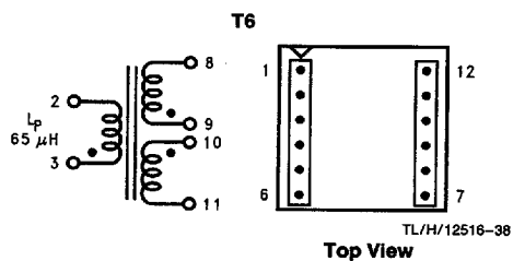
FIGURE 20. Coilcraft Q4438-B (Surface Mount)
