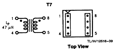
FIGURE 21. Pulse PE-68482
