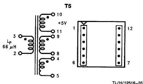
FIGURE 17. Coilcraft Q4437-B (Surface Mount)
