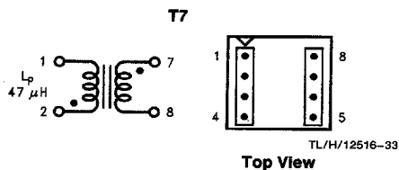
FIGURE 15. Coilcraft S6000-A
