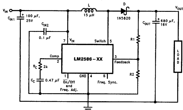
FIGURE 2. LM2586-12 and LM2586-ADJ
