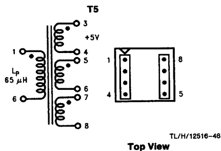
FIGURE 26. Renco RL-5532
