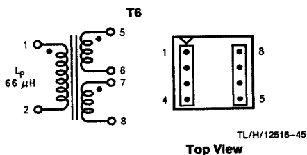
FIGURE 25. Renco RL-5533
