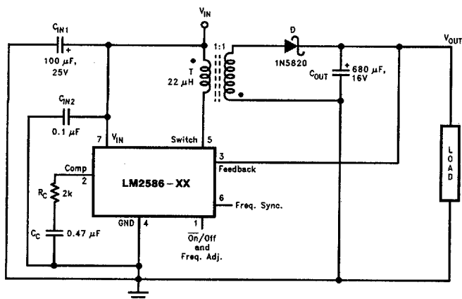
FIGURE 1. LM2586-3.3 and LM2586-5.0
