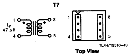
FIGURE 24. Renco RL-5751
