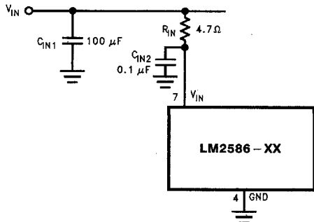
FIGURE 44. Input Line Filter
