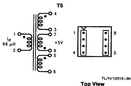
FIGURE 18. Coilcraft Q4338-B
