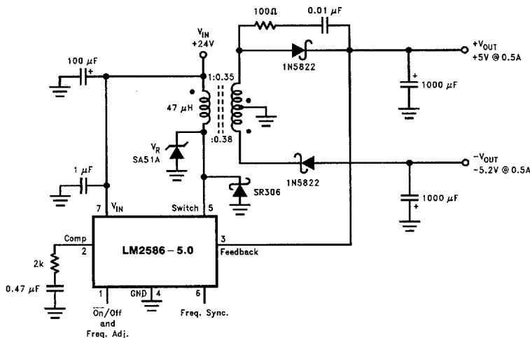
FIGURE 43. Flyback Regulator
