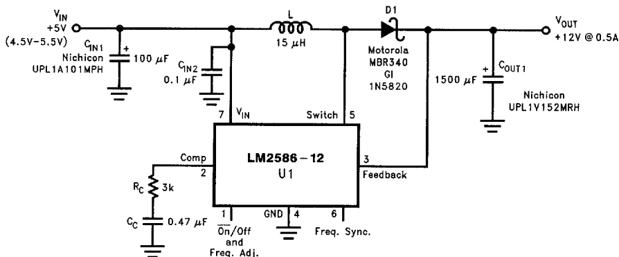
FIGURE 33. +5V to +12V Boost Regulator
