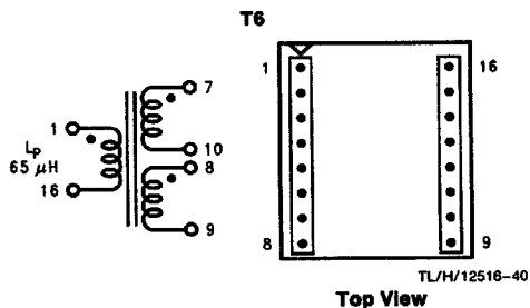
FIGURE 22. Pulse PE-68414 (Surface Mount)
