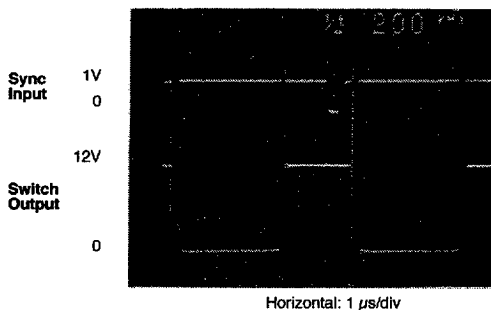
FIGURE 41. Waveforms of a Synchronized 12V Boost Regulator
