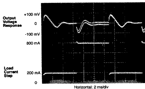
FIGURE 32. V_{OUT} Response to Load Current Step
