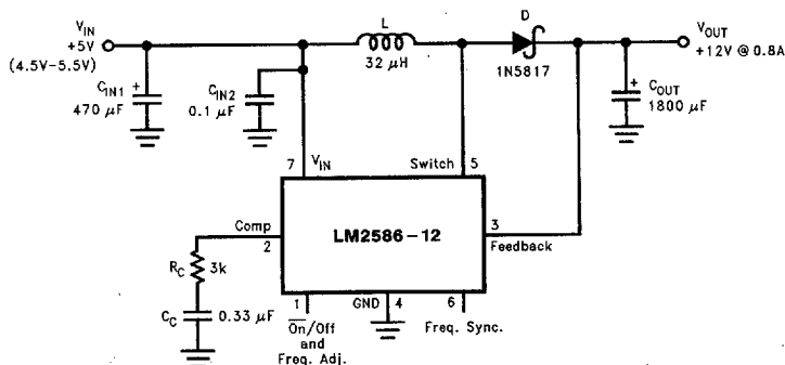
FIGURE 30. 12V Boost Regulator
