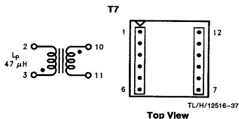
FIGURE 19. Coilcraft S6057-A (Surface Mount)
