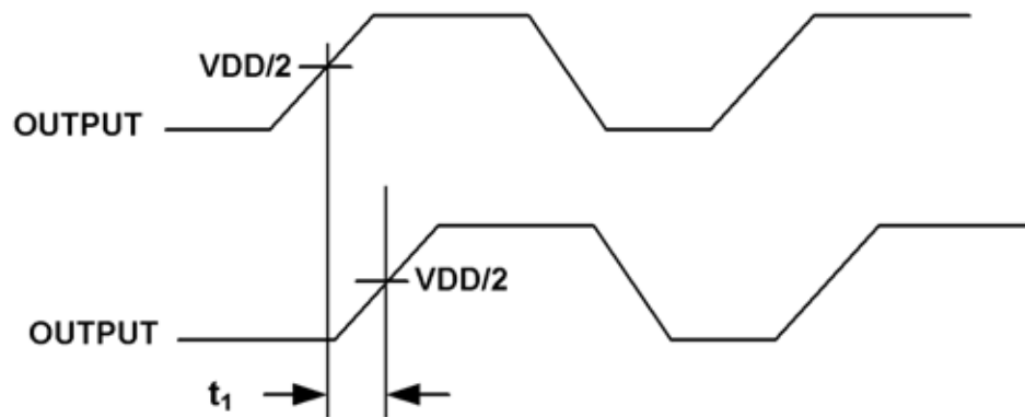
Figure 2. Output to Output Skew
