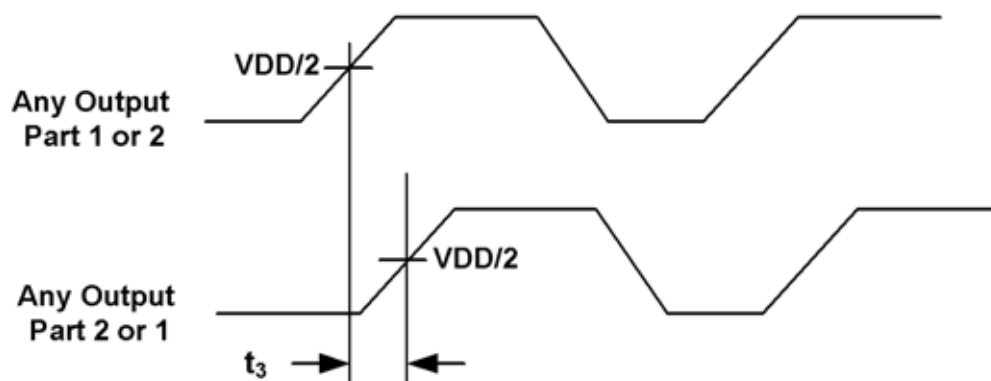
Figure 4. Part-to-Part Skew
