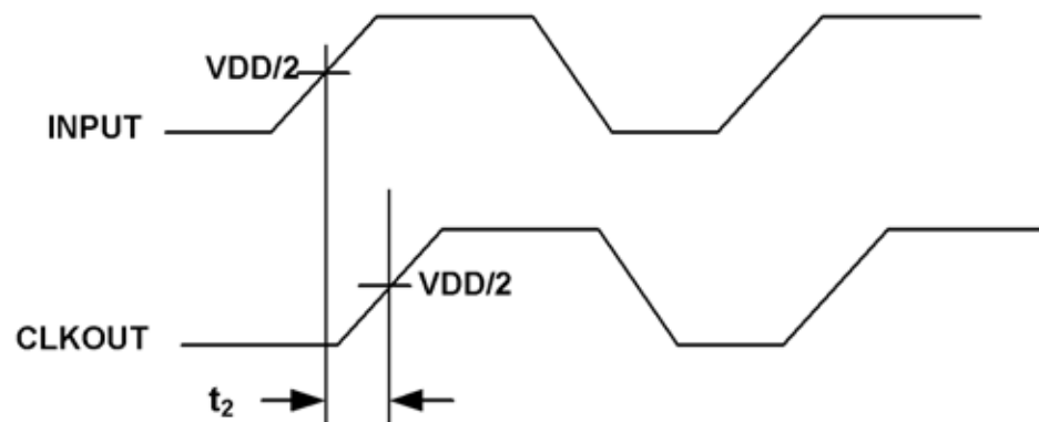
Figure 3. Input to Output Skew
