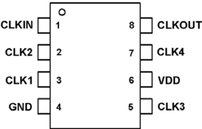
Figure 5. 8-Pin SOIC
