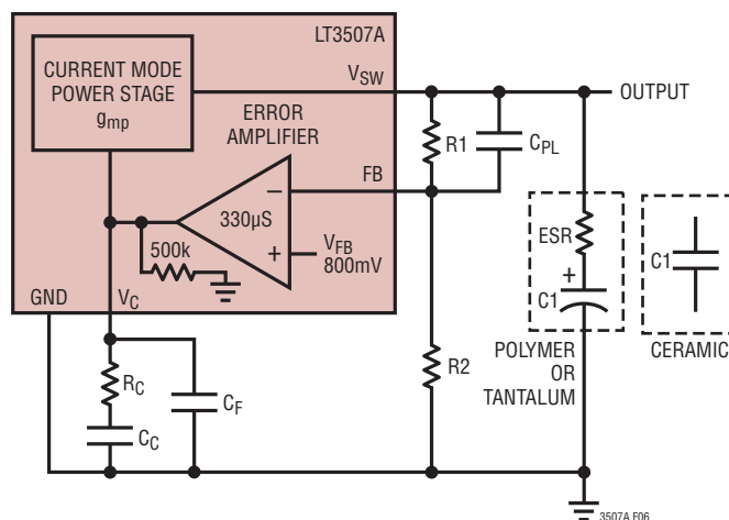
Figure 6. Loop Response Model
