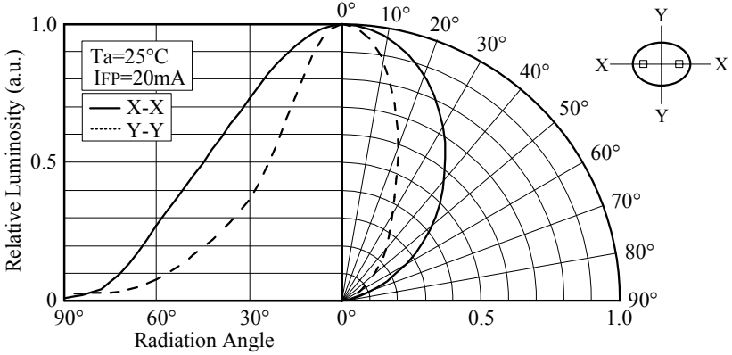
■ Directivity
