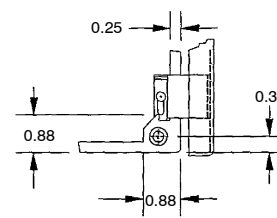
Hinge Detail
