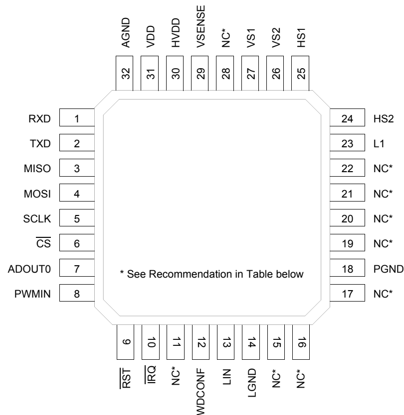
Figure 3. 33910 Pin Connections
