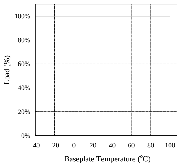
Derating Curve
