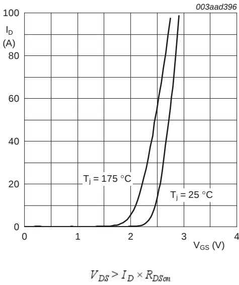
Fig 8. Transfer characteristics: drain current as a function of gate-source voltage; typical values
