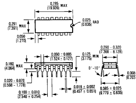
16 Lead Cerdip
