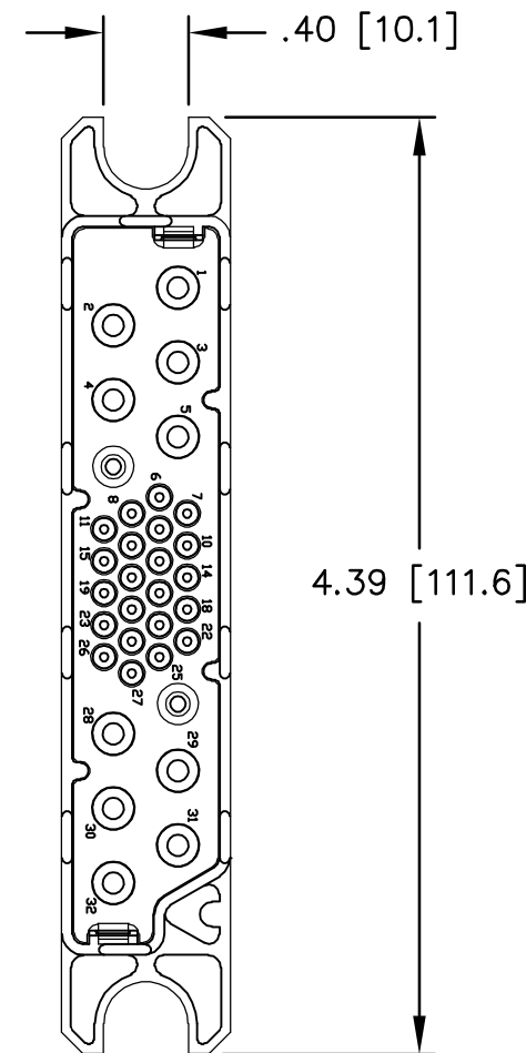
REAR VIEW (PIN CONTACT INSERTION SIDE)
