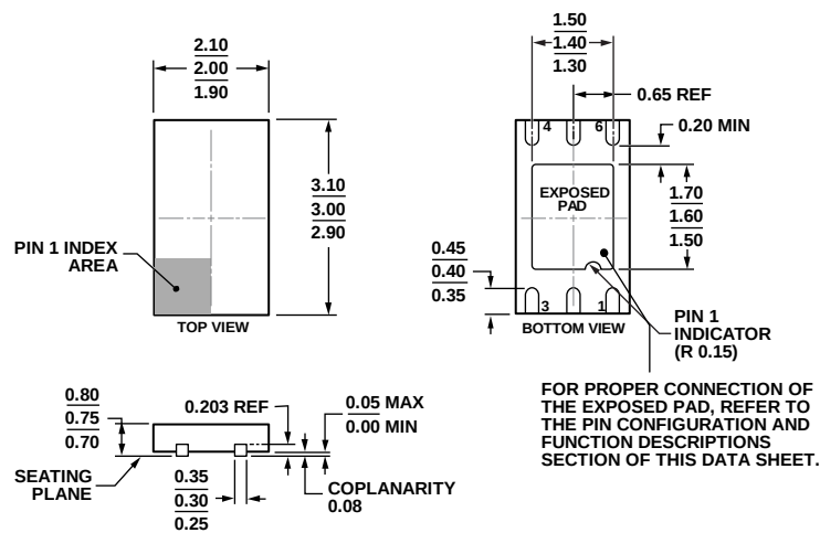
Figure 55. 6-Lead Lead Frame Chip Scale Package [LF CSP_WD] 2.00 × 3.00 mm Body, Very Very Thin, Dual Lead (CP-6-5)
