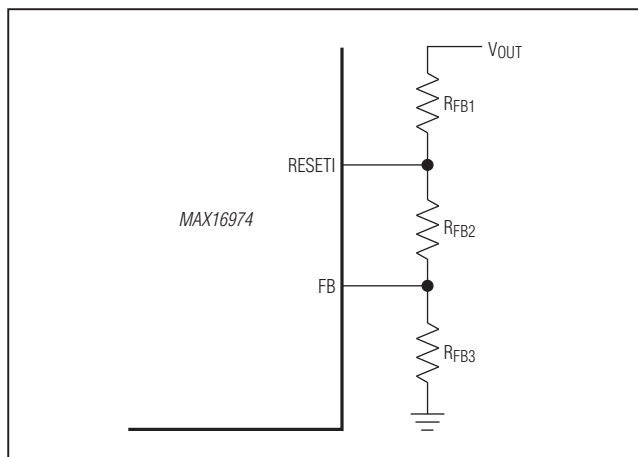
Figure 3. Output Voltage/Reset Threshold Resistive Divider Network
