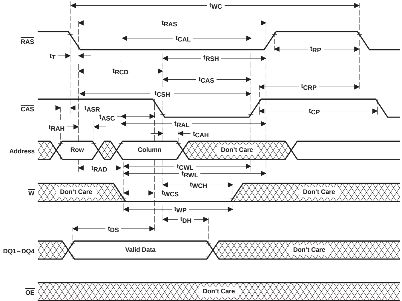
Figure 4. Early-Write-Cycle Timing
