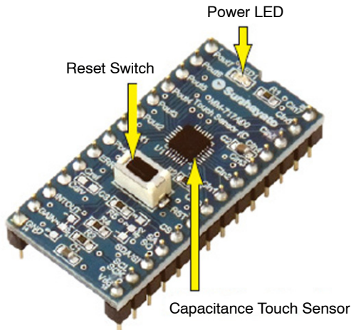
Figure 6. LC717A00ARGPGEVB
