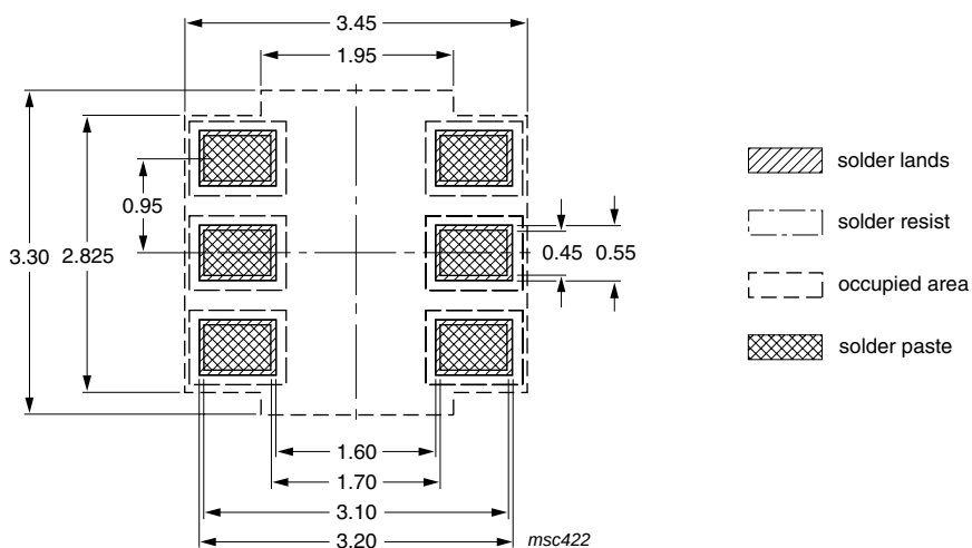
Fig 26. Reflow soldering footprint
