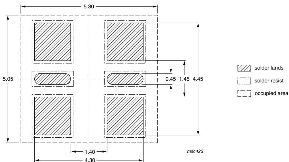
Fig 26. Reflow soldering footprint
