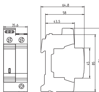
OVR T2 1N 40-275 P TS OVR T2 1N 40-275s P TS OVR T2 1N 70-275s P TS
