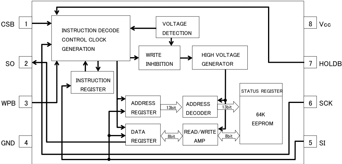
Figure 3. Block Diagram
