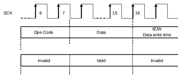
Figure 43. WPB valid timing (At inputting WRSR command)
