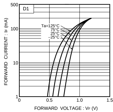
Fig.5 Forward characteristics
