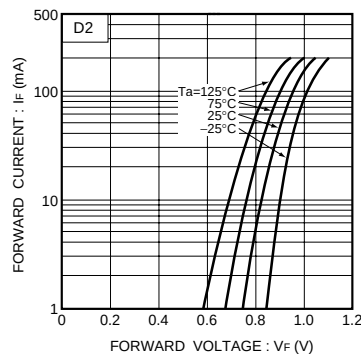
Fig.6 Forward characteristics
