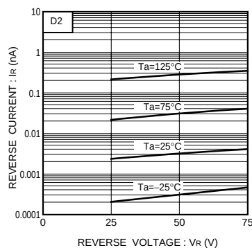
Fig.8 Reverse characteristics
