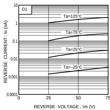
Fig.7 Reverse characteristics
