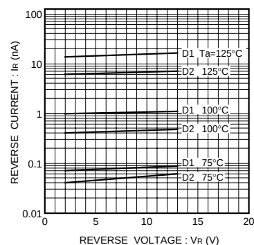
Fig.3 Reverse characteristics
