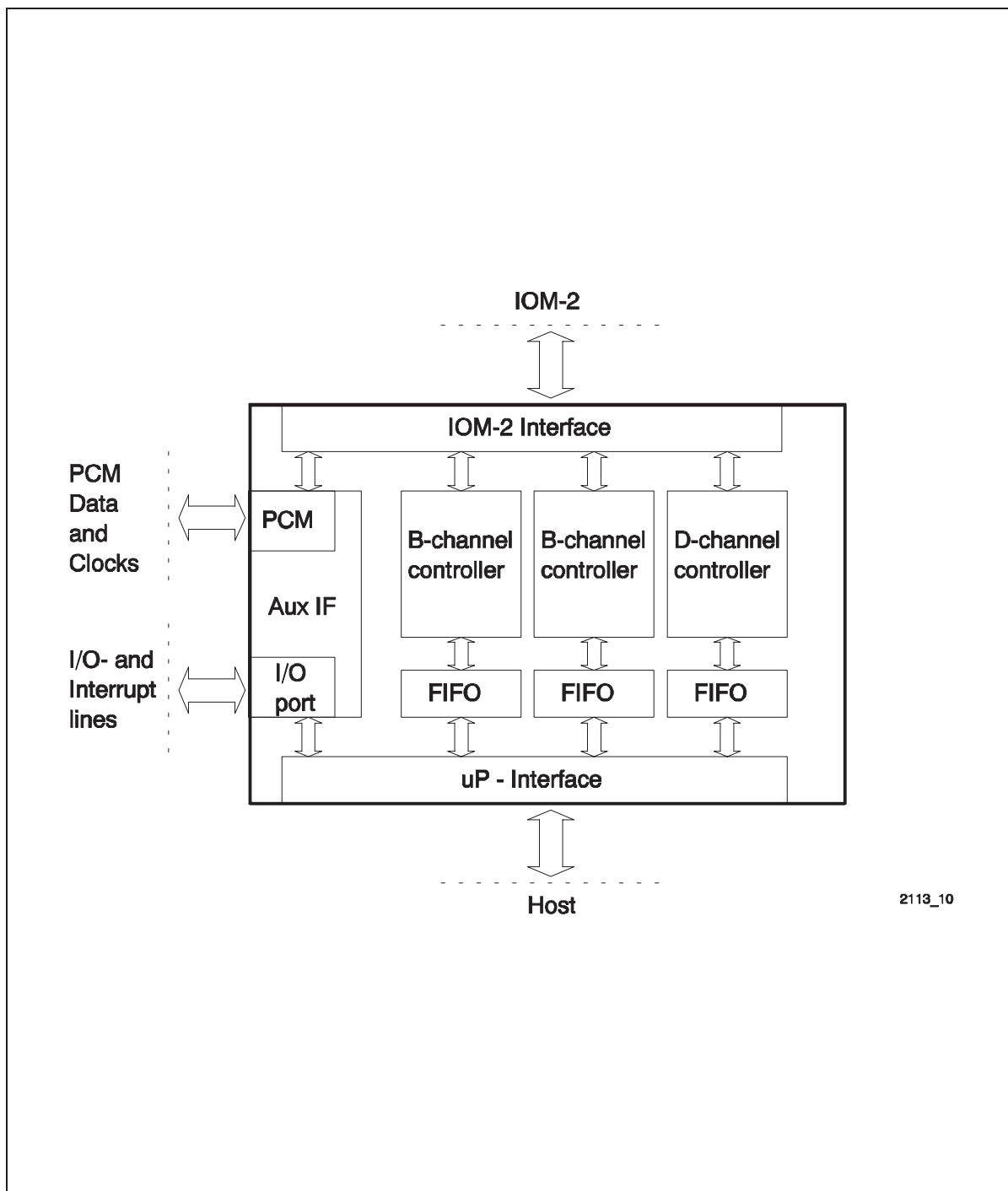
Figure 3 Block Diagram
