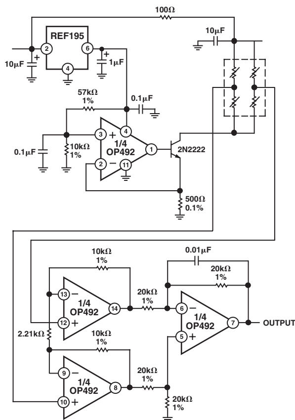
Figure 12. A Low Power, Strain Gage Circuit
