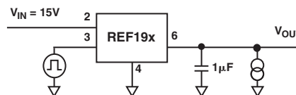
TPC 11b. SLEEP Response Time Measurement Circuit
