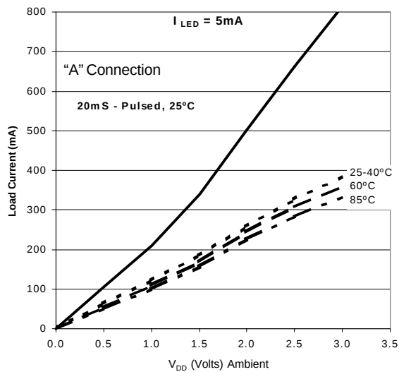
Figure 3. Typical On-Characteristics
