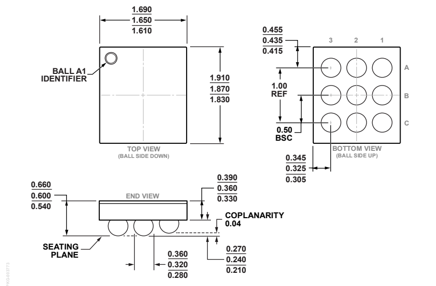
Figure 42. 9-Ball Wafer Level Chip Scale Package [WLCSP] (CB-9-6)
