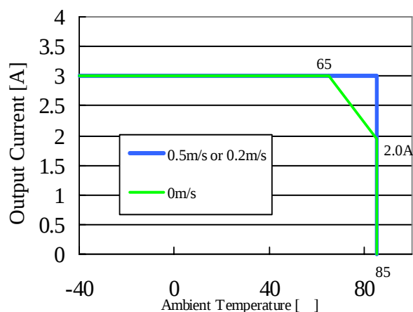
MPD6D105S ( V_o=2.0V )
