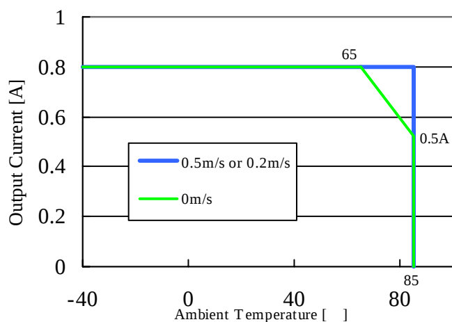
MPD6D101S ( V_o=12V )
