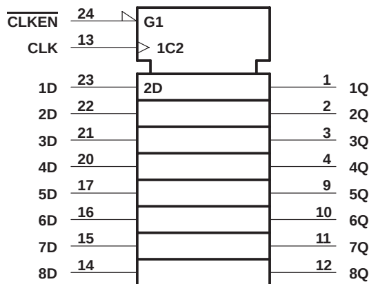
logic symbol†
