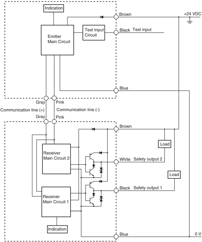
Entire Circuit Diagram
