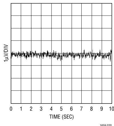
LTC1657L 0.1Hz to 10Hz Voltage Noise
