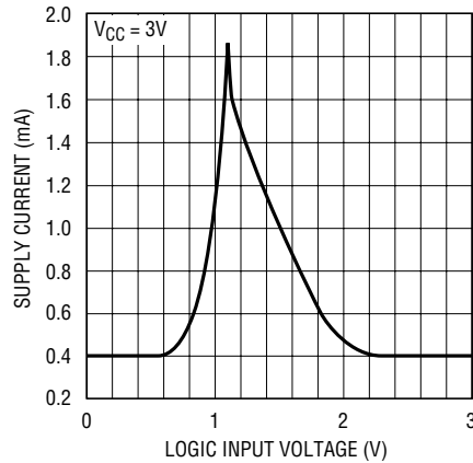
LTC1657L Supply Current vs Logic Input Voltage
