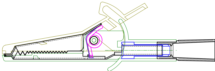
113387 ADAPTER MOULDING
