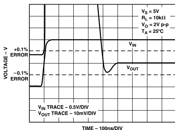
TPC 47. Settling Time
