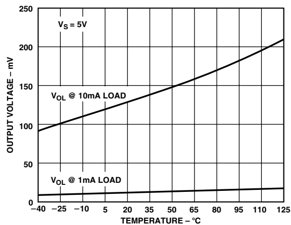
TPC 15. Output Voltage Swing vs. Temperature
