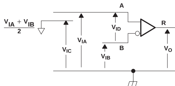
Figure 9. Voltage Definitions
