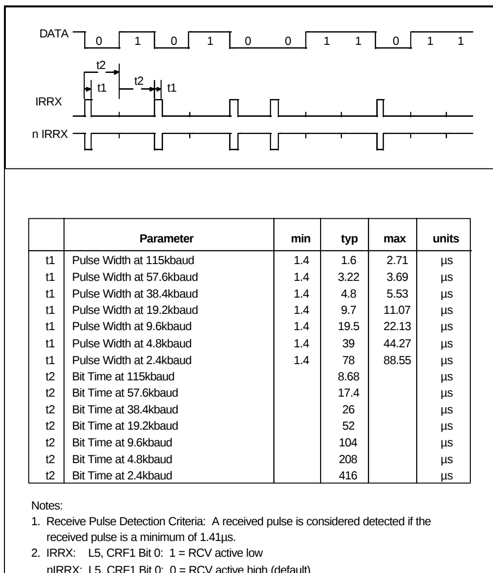
FIGURE 20 - IrDA RECEIVE TIMING
