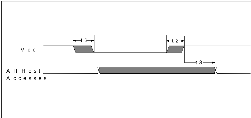
FIGURE 4 - POWER-UP TIMING
