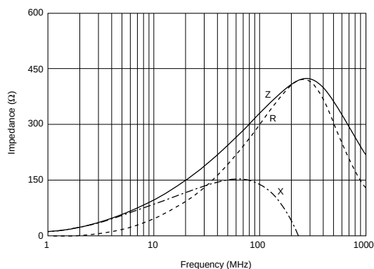
BLM18AG331SN1
