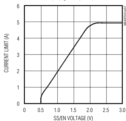
OUTPUT CURRENT LIMIT vs. SS/EN VOLTAGE
