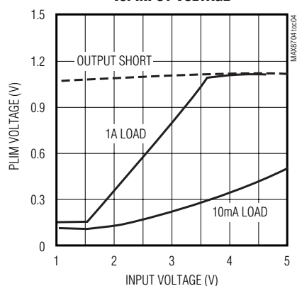
PLIM VOLTAGE vs. INPUT VOLTAGE
