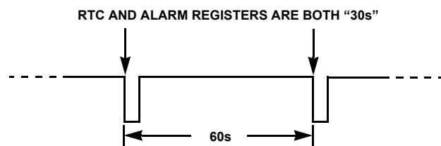
FIGURE 5. \overline{\text{IRQ}} WAVEFORM
