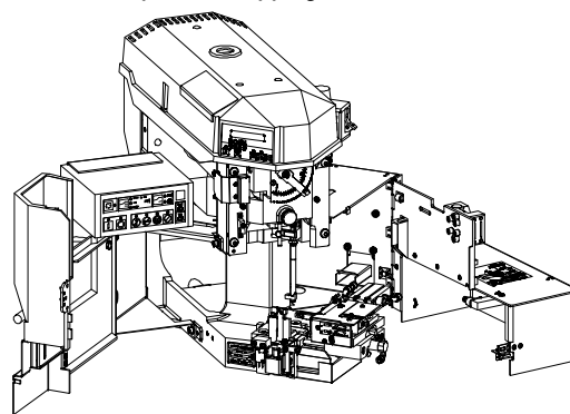
AMP-O-LECTRIC Model "G" Terminating Machine 354500-[ ] with Optional Stripping Module
