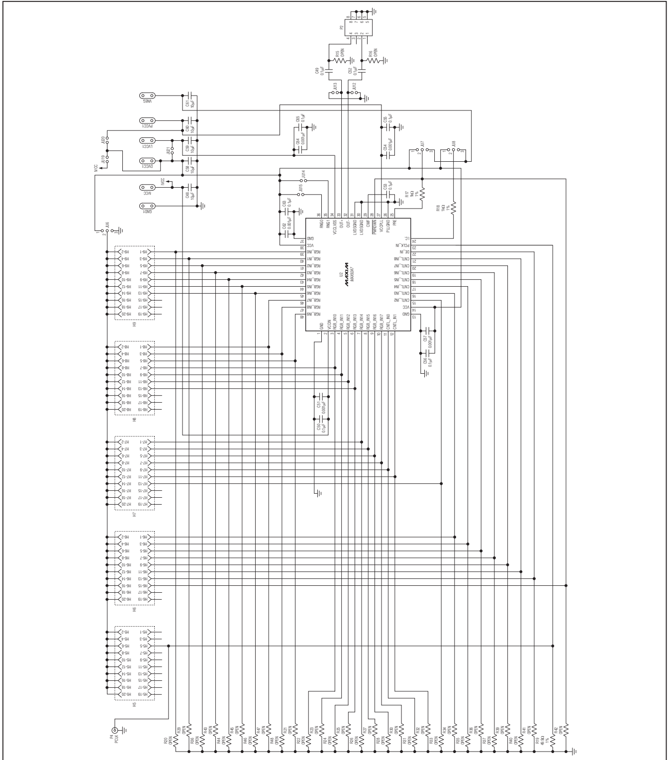
Figure 1b. MAX9247/MAX9248 EV Kit Schematic (Sheet 2 of 2)
