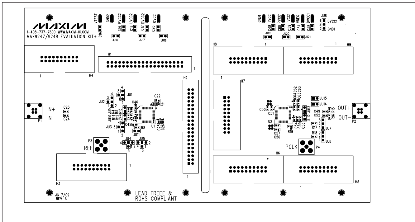
Figure 2. MAX9247/MAX9248 EV Kit Component Placement Guide—Component Side
