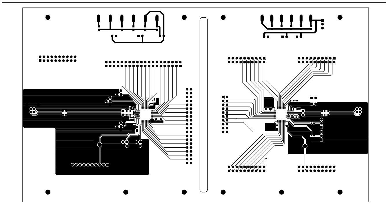
Figure 3. MAX9247/MAX9248 EV Kit PCB Layout—Component Side
