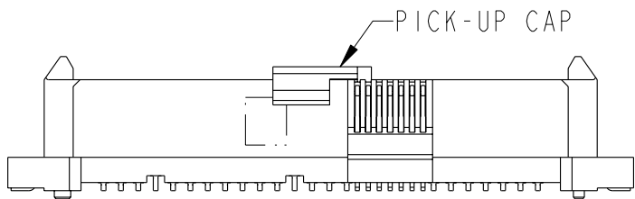
PART WITH PICK-UP CAP, SEE NOTE ④
