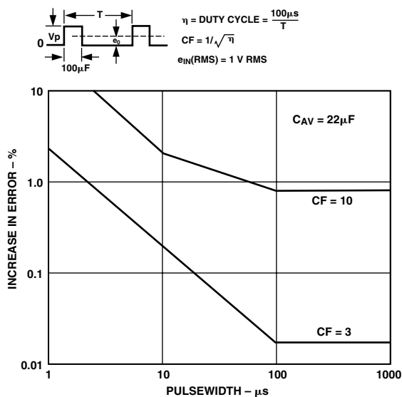
Figure 11. AD637 Error vs. Pulsewidth Rectangular Pulse
