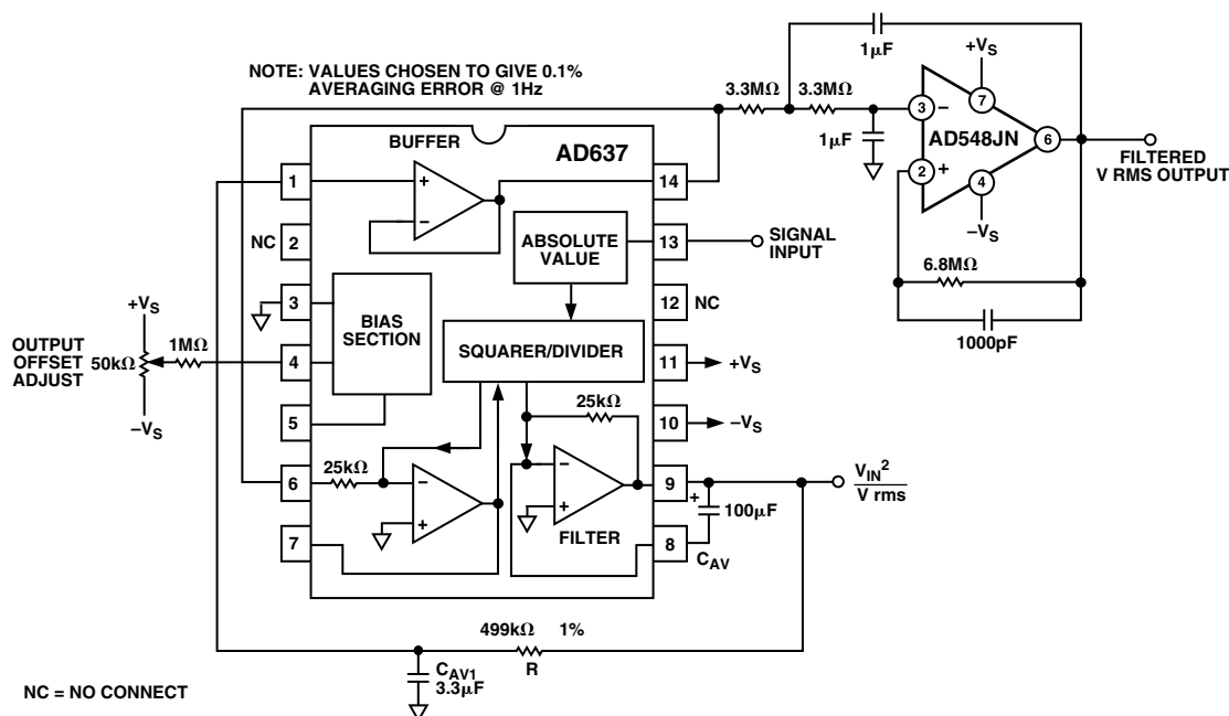
Figure 15. AD637 as a Low Frequency RMS Converter
