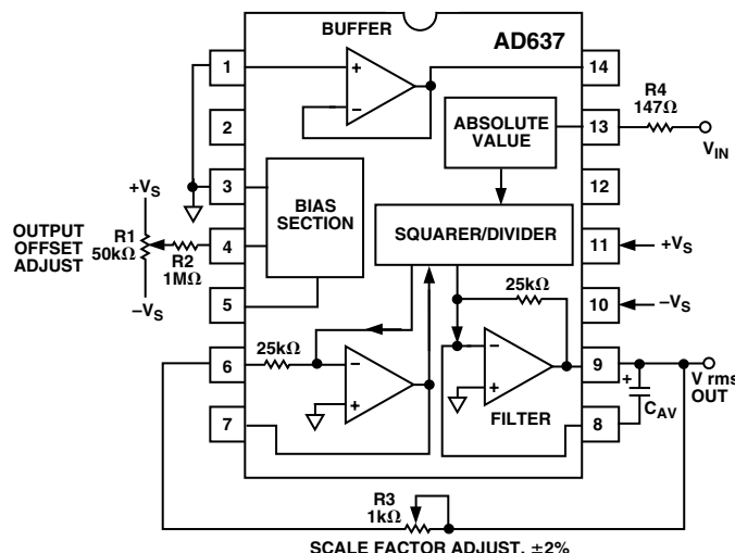
Figure 5. Optional External Gain and Offset Trims
