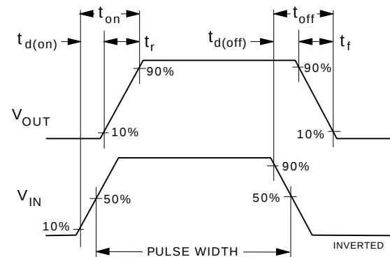
Figure 12. Switching Waveforms.
