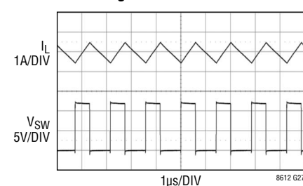
Switching Waveforms
