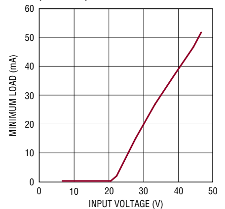
Minimum Load to Full Frequency (SYNC Hi)
