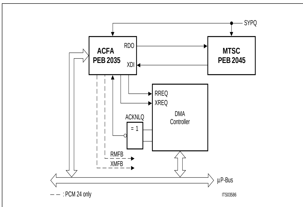
Figure 16 Connection to a DMA Controller
