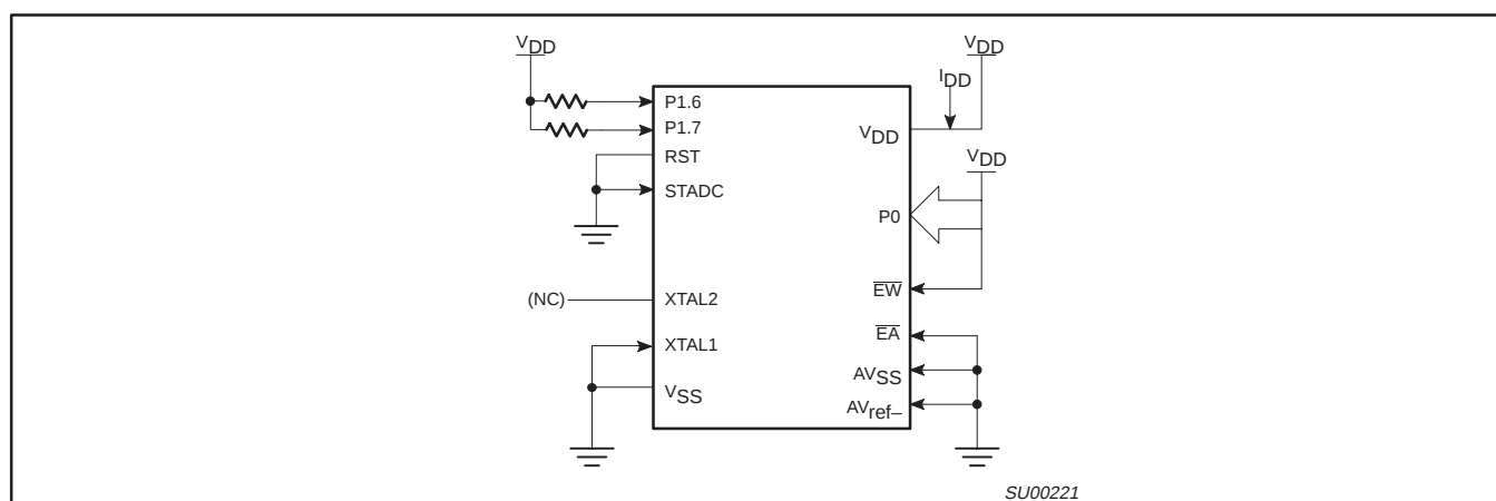
Figure 60. I_{DD} Test Condition, Power Down Mode All other pins are disconnected. V_{DD} = 2\text{V to } 5.5\text{V}^3
