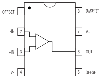
8 LEAD
