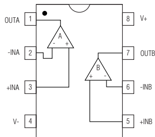
8 LEAD
