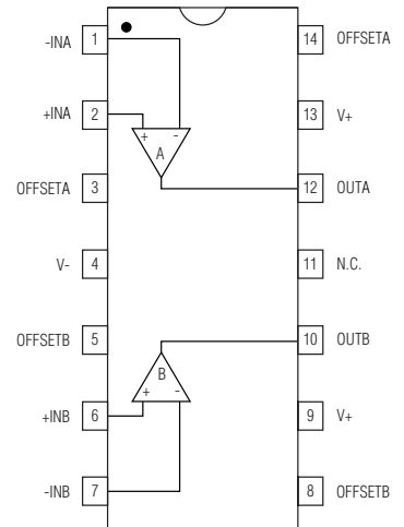
14 LEAD
