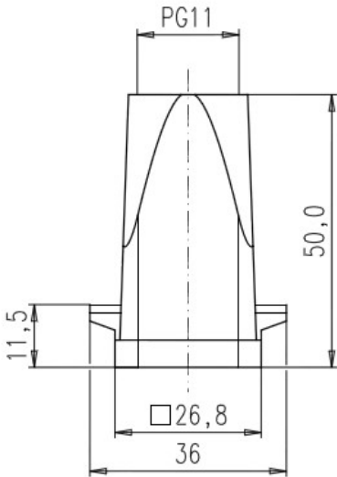
Drawing Dimensions in mm (Inch) 11.01.2013
