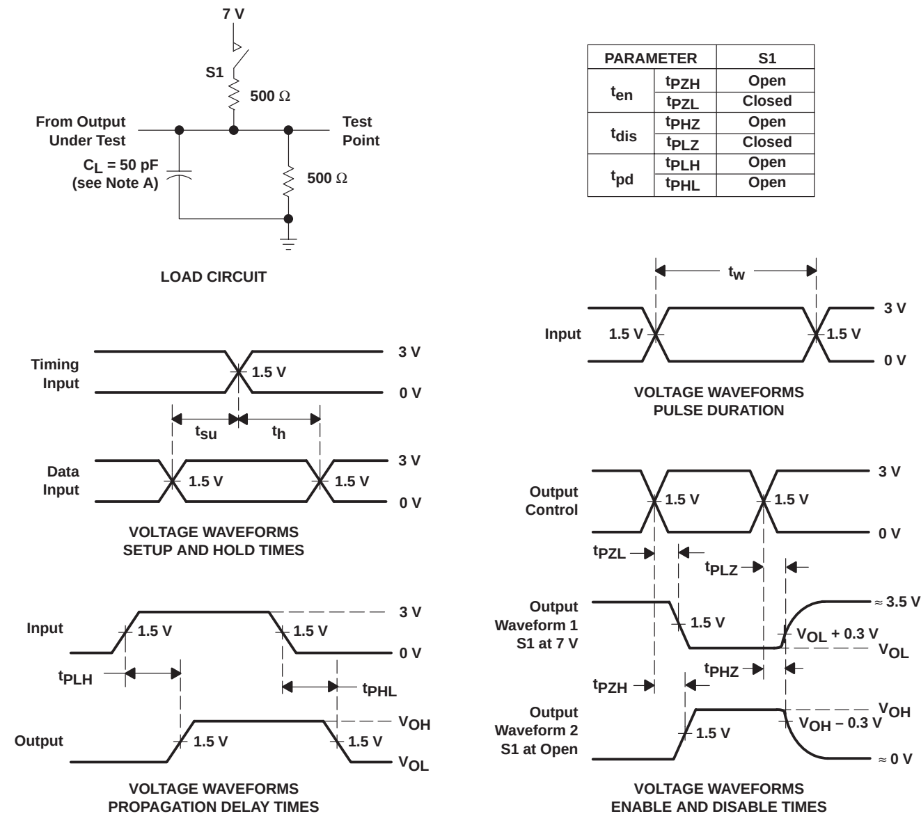
Figure 3. Load Circuit and Voltage Waveforms
