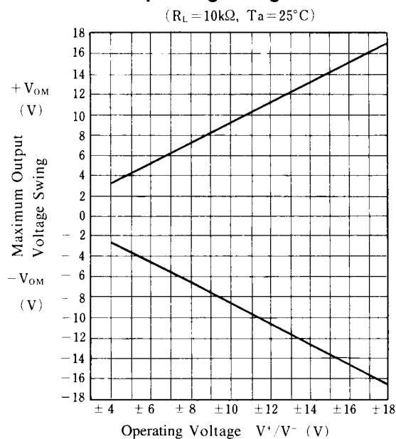
Maximum Output Voltage Swing vs. Operating Voltage
