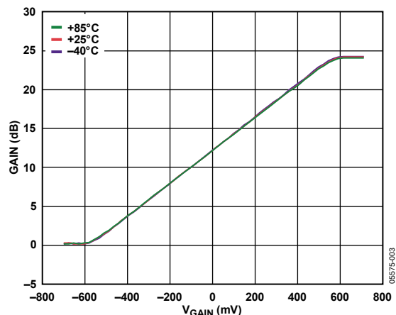
Figure 3. Gain vs. V_{GAIN} at Three Temperatures (See Figure 44)
